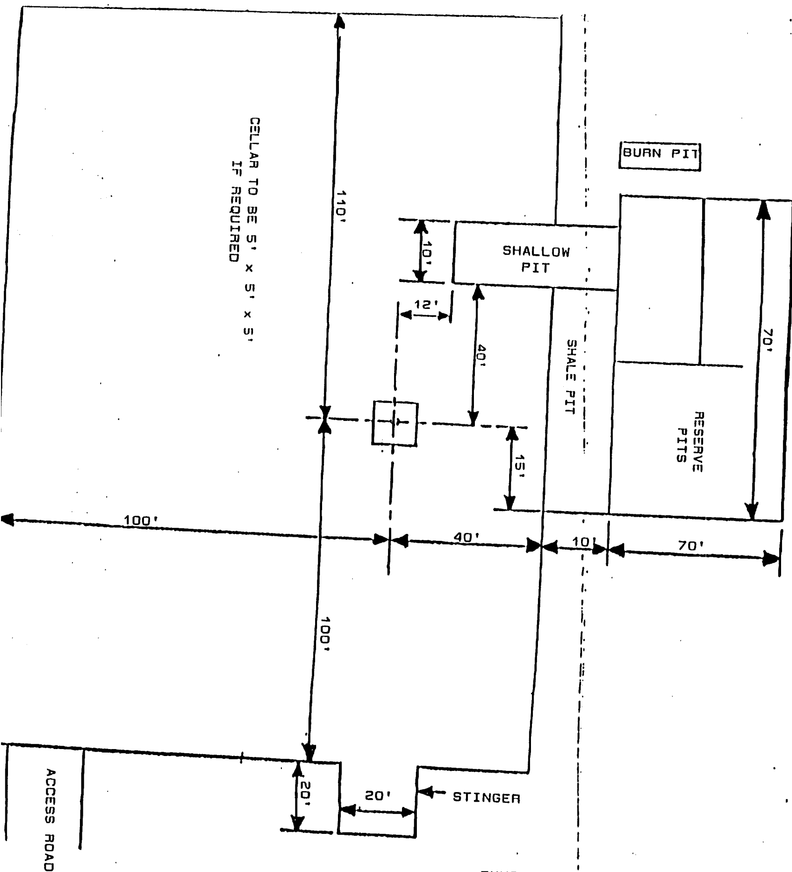
EXHIBIT "D" Socorro Petroleum Company Turner "B" #83 Rig Layout
