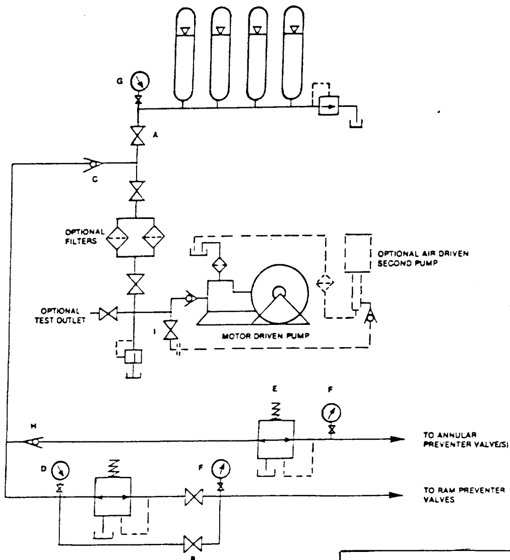
EXHIBIT "E-1" CHOLE MANIFOLD & CLOSING UNIT
