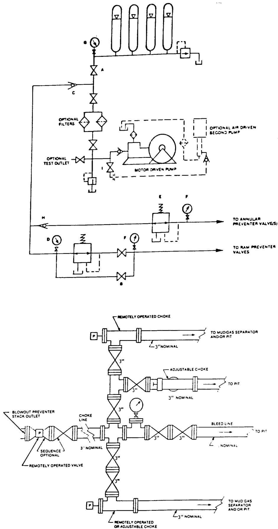
FIGURE K4-3. Typical choke manifold assembly for 10M and 15M rated
