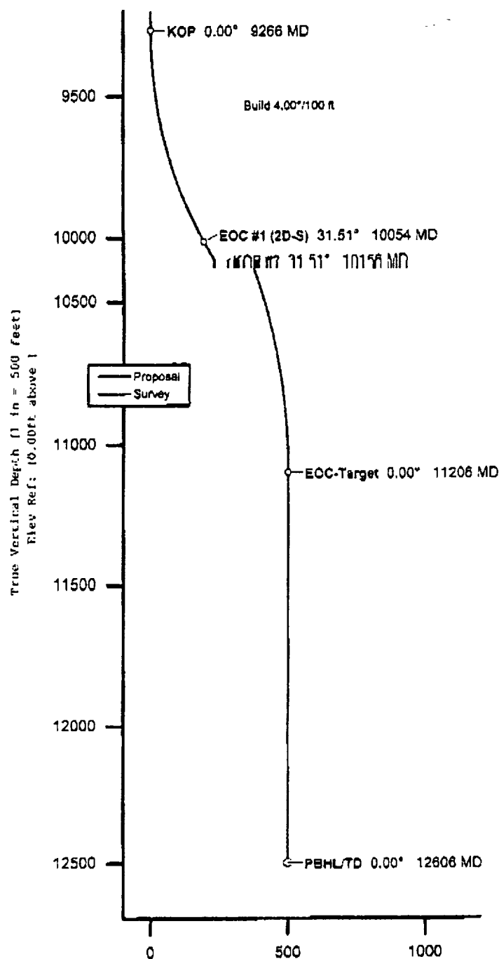
Vertical Section View
