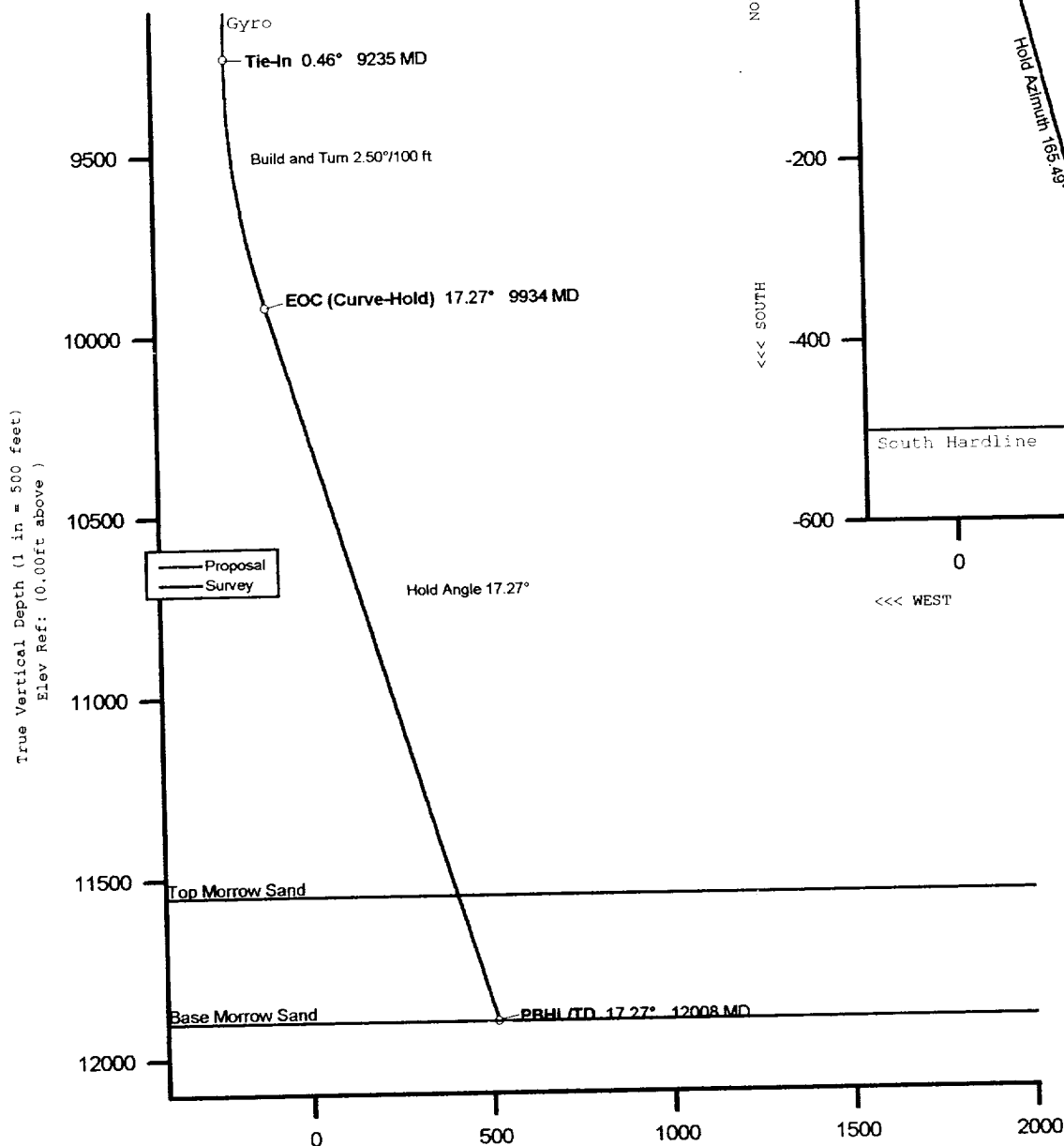
Vertical Section View
