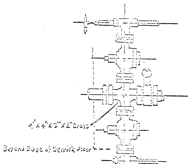
Choke Manifold
