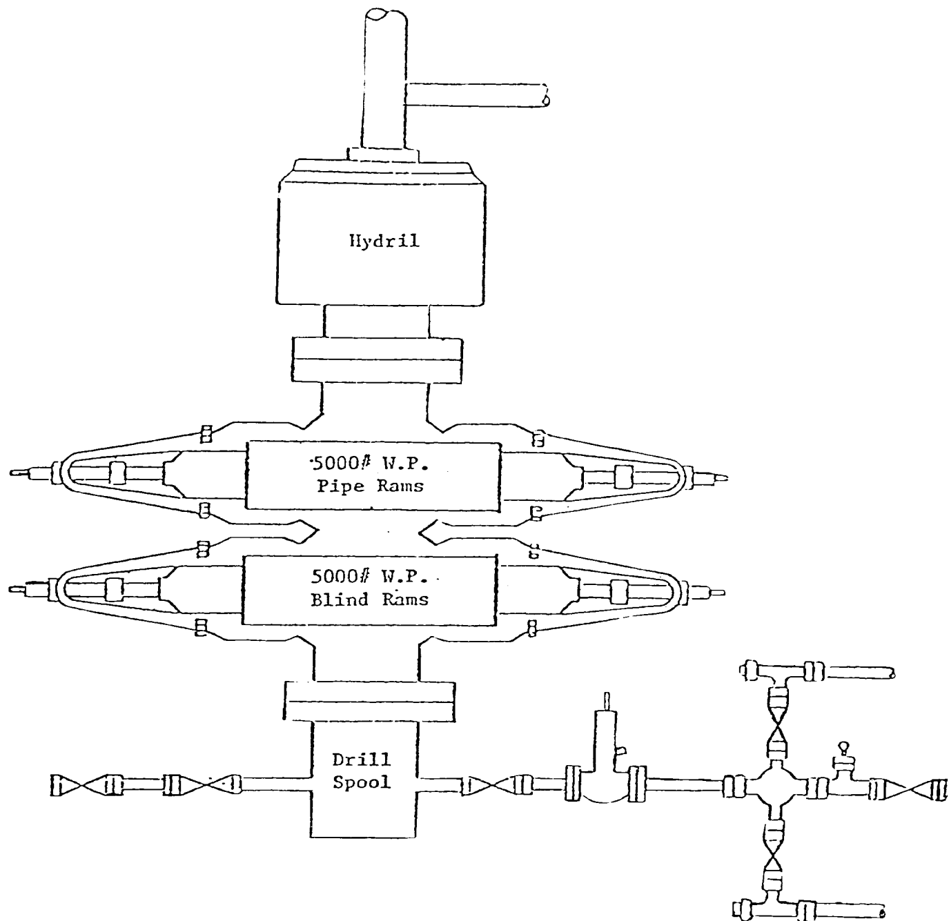
Blowout Preventer Schematic 5000 psi Working Pressure Series 1500 Flange Connections
