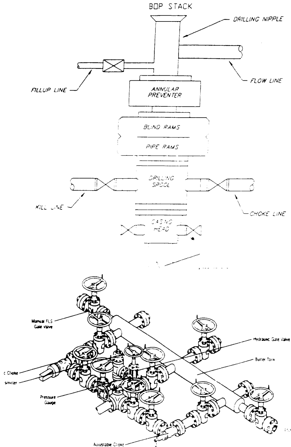
Typical Choke Manifold Designed for Land Drilling Applications
