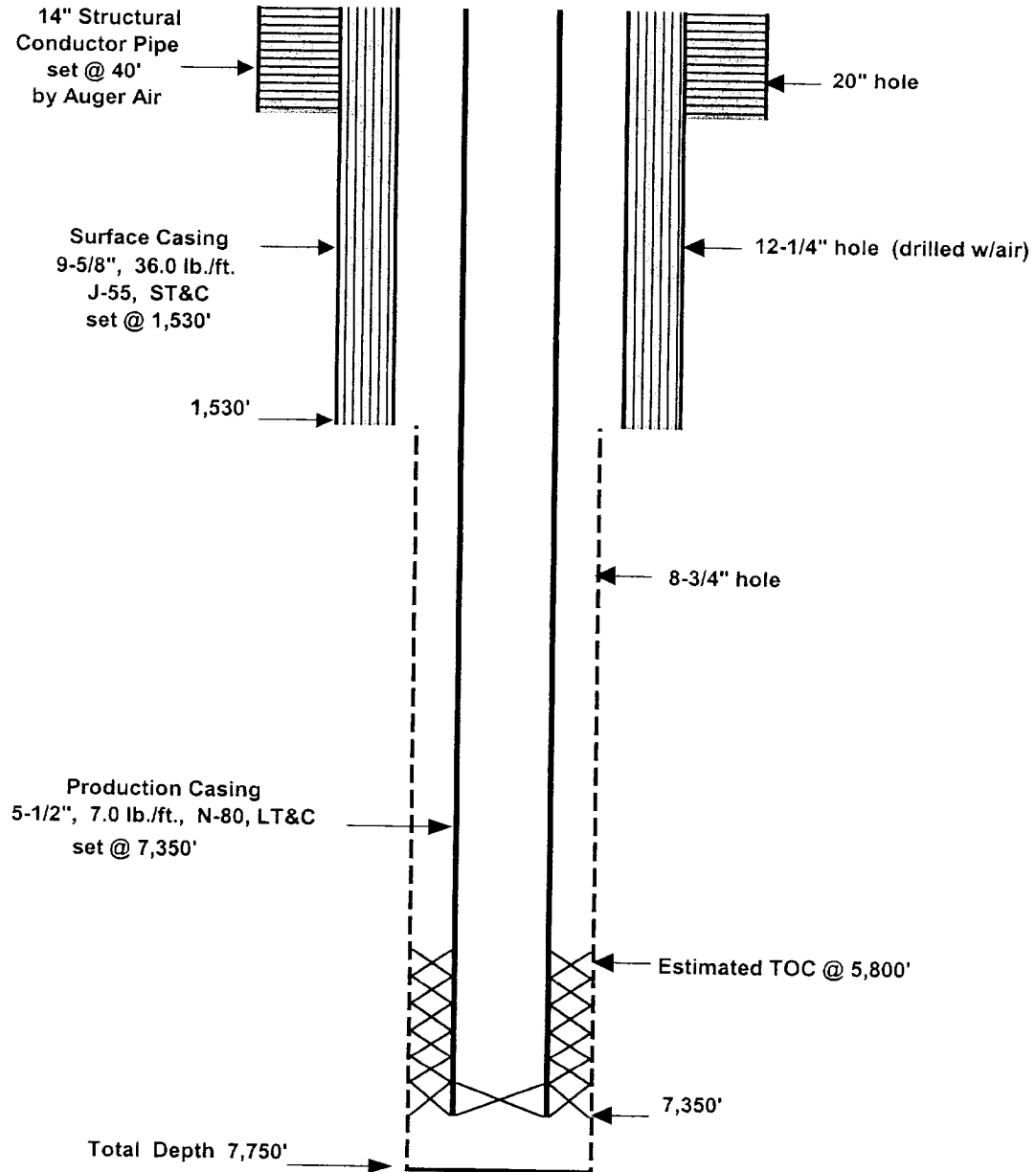
Current Wellbore Schematic
