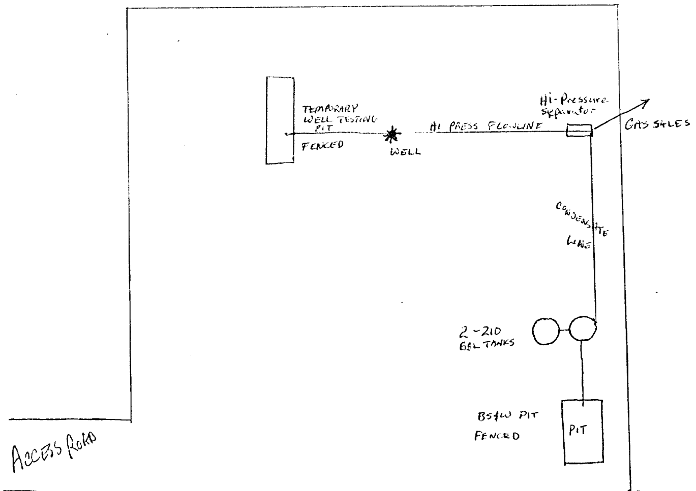
PROPOSED TANK BATTERY LAYOUT
