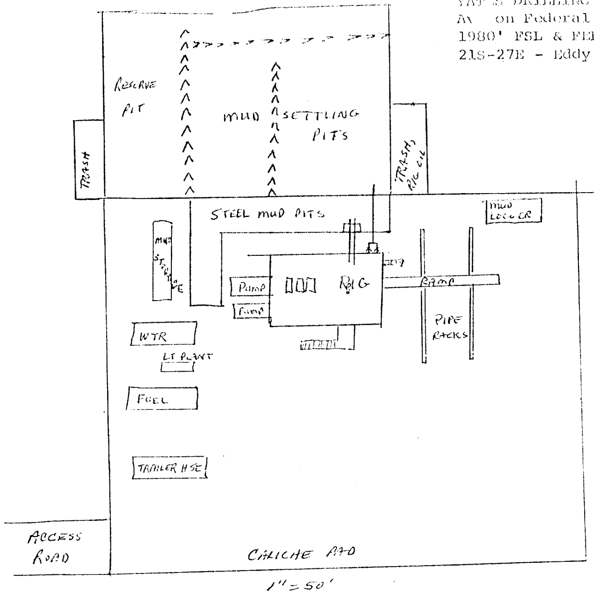
PROPOSED DRILLING WELL SITE
