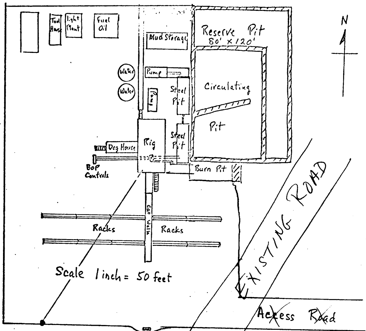
Drilling Rig Layout
