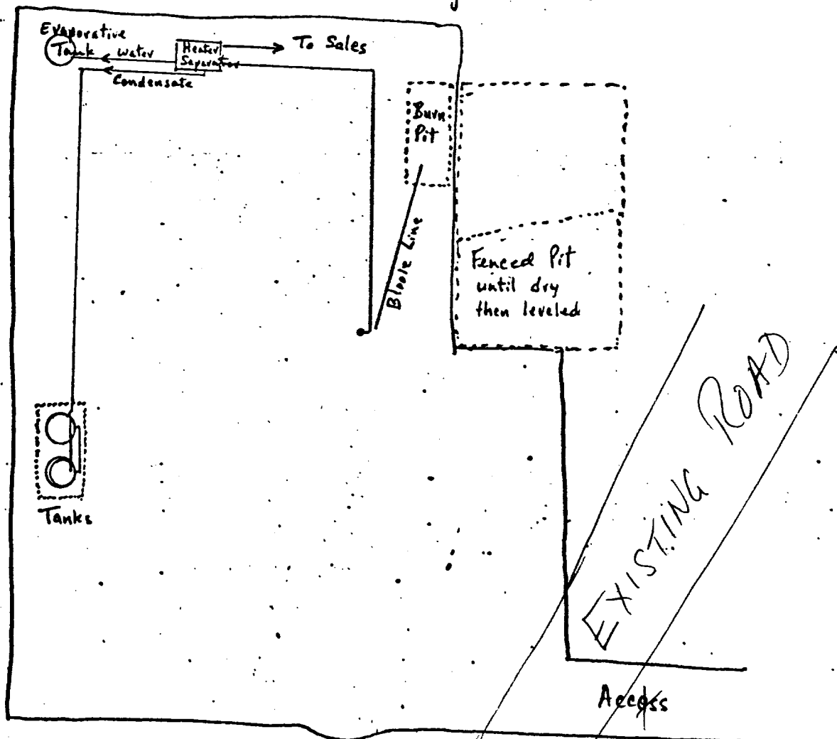
Tank Battery layout
