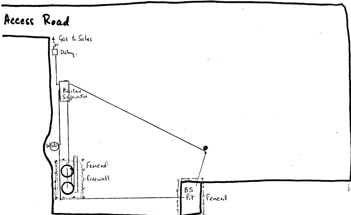
Tank Battery layout
