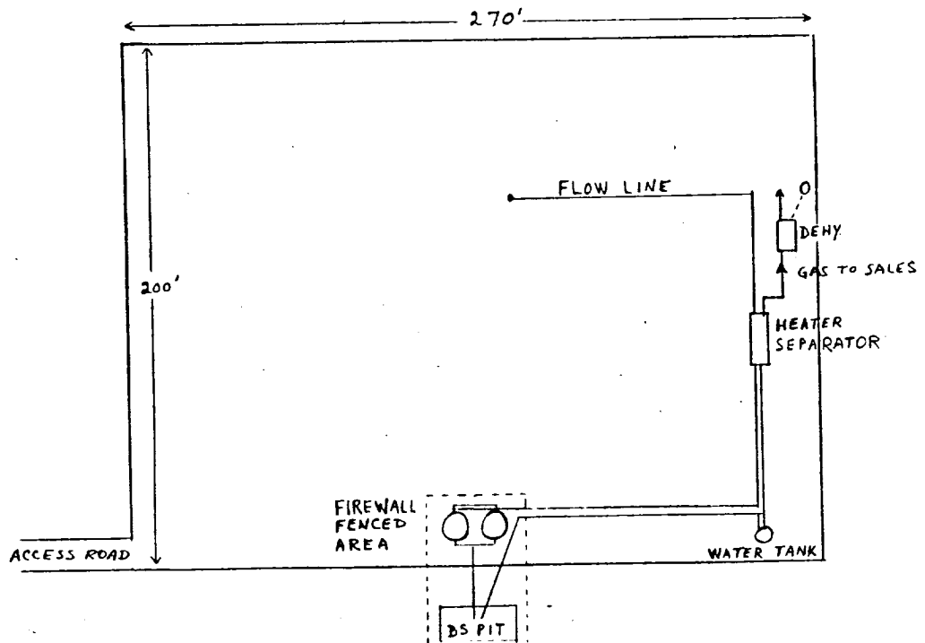
TANK BATTERY LAYOUT
