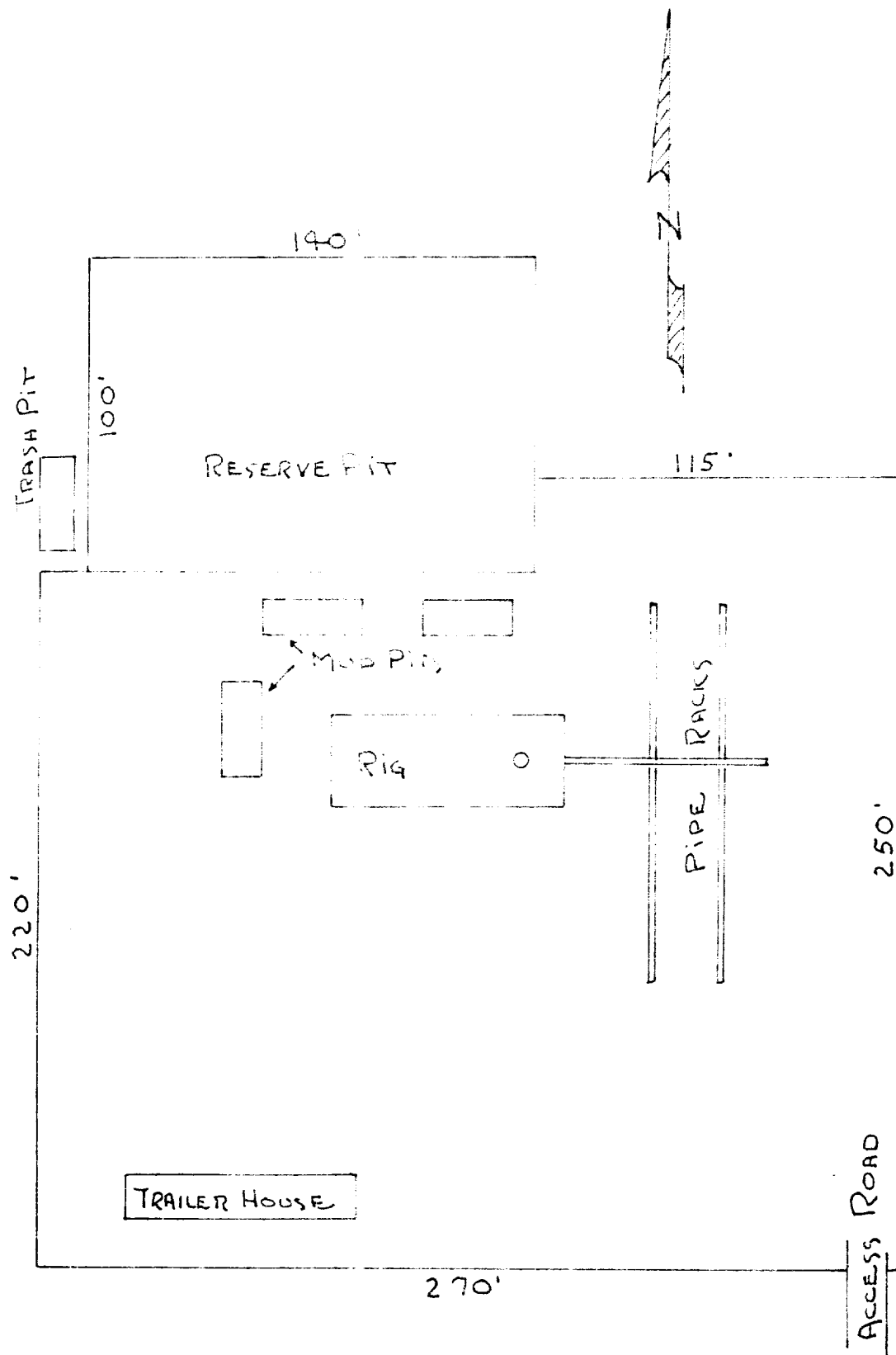
EXHIBIT "C" DRILLING RIG LAYOUT SCALE: 1" = 50'
