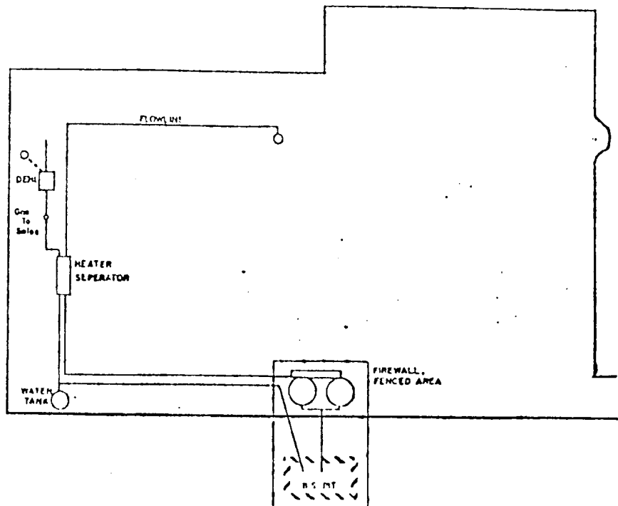
TANK BATTERY LAYOUT
