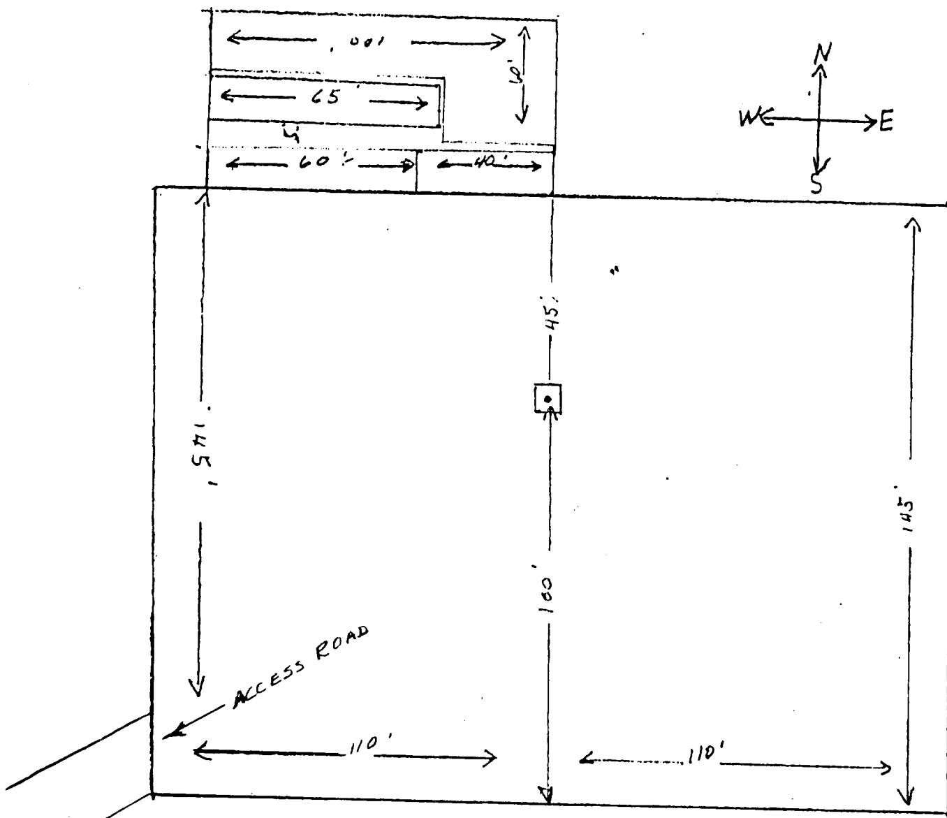
EXHIBIT "D" CHI OPERATING, INC. Azotea Federal, Well No. 1 Pad & Pit Layout
