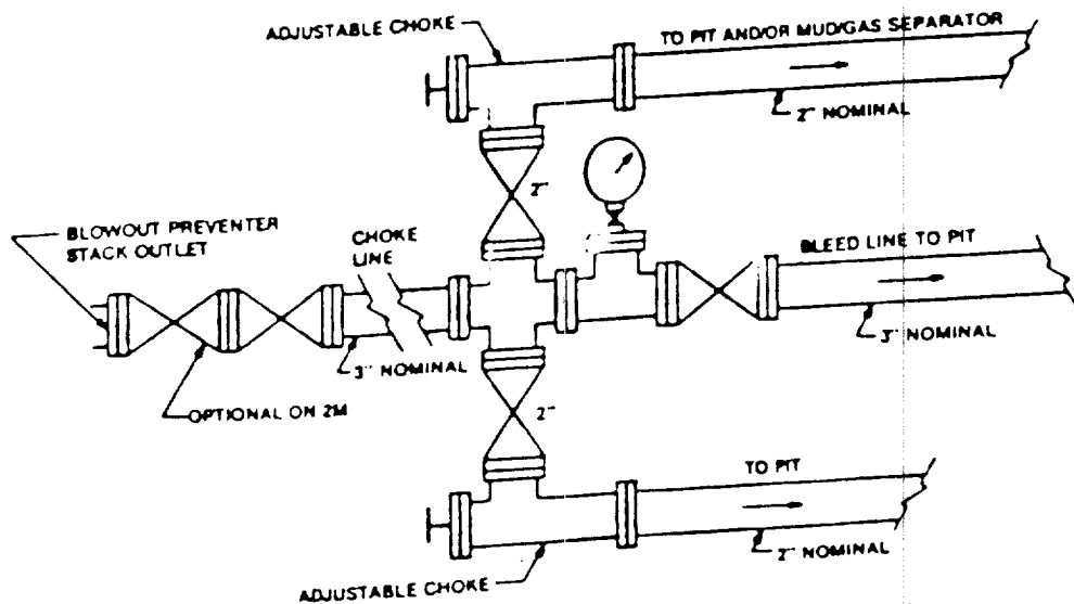
FIGURE K4-1. Typical choke manifold assembly for 2M and 3M wellheads working pressure service — surface installation.
