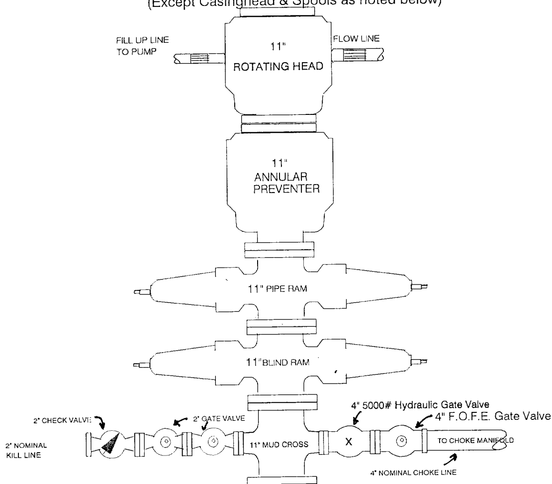
WELLHEAD EQUIPMENT: Intermediate Profile 2,625' - 11,200'
