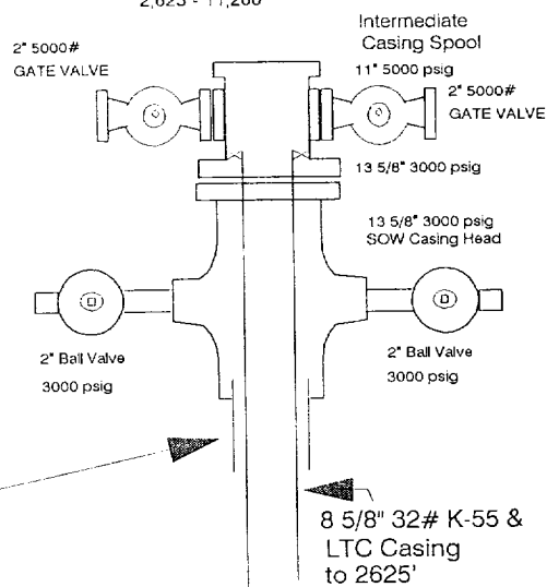
WELLHEAD EQUIPMENT: Intermediate Profile 2,625' - 11,200'
