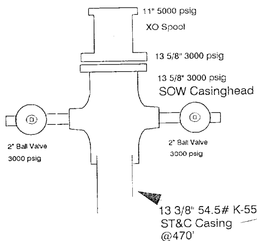
WELLHEAD EQUIPMENT: Surface Profile: 475' - 2,625'
