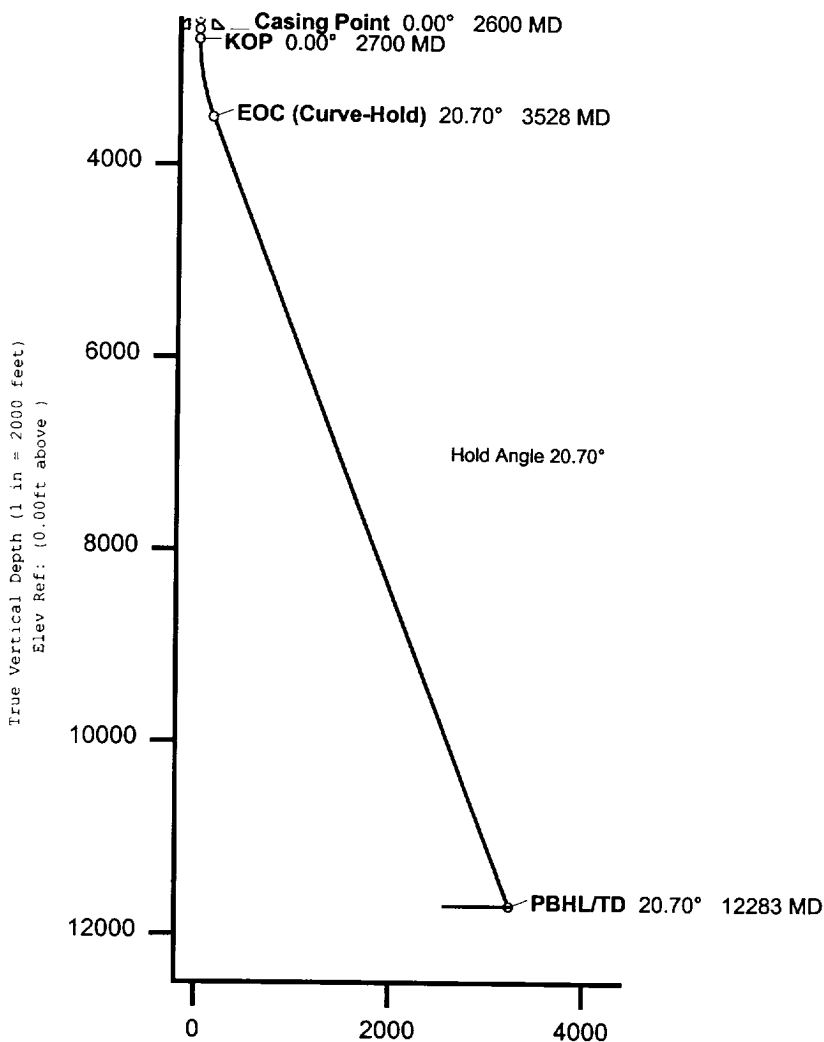
Vertical Section View
