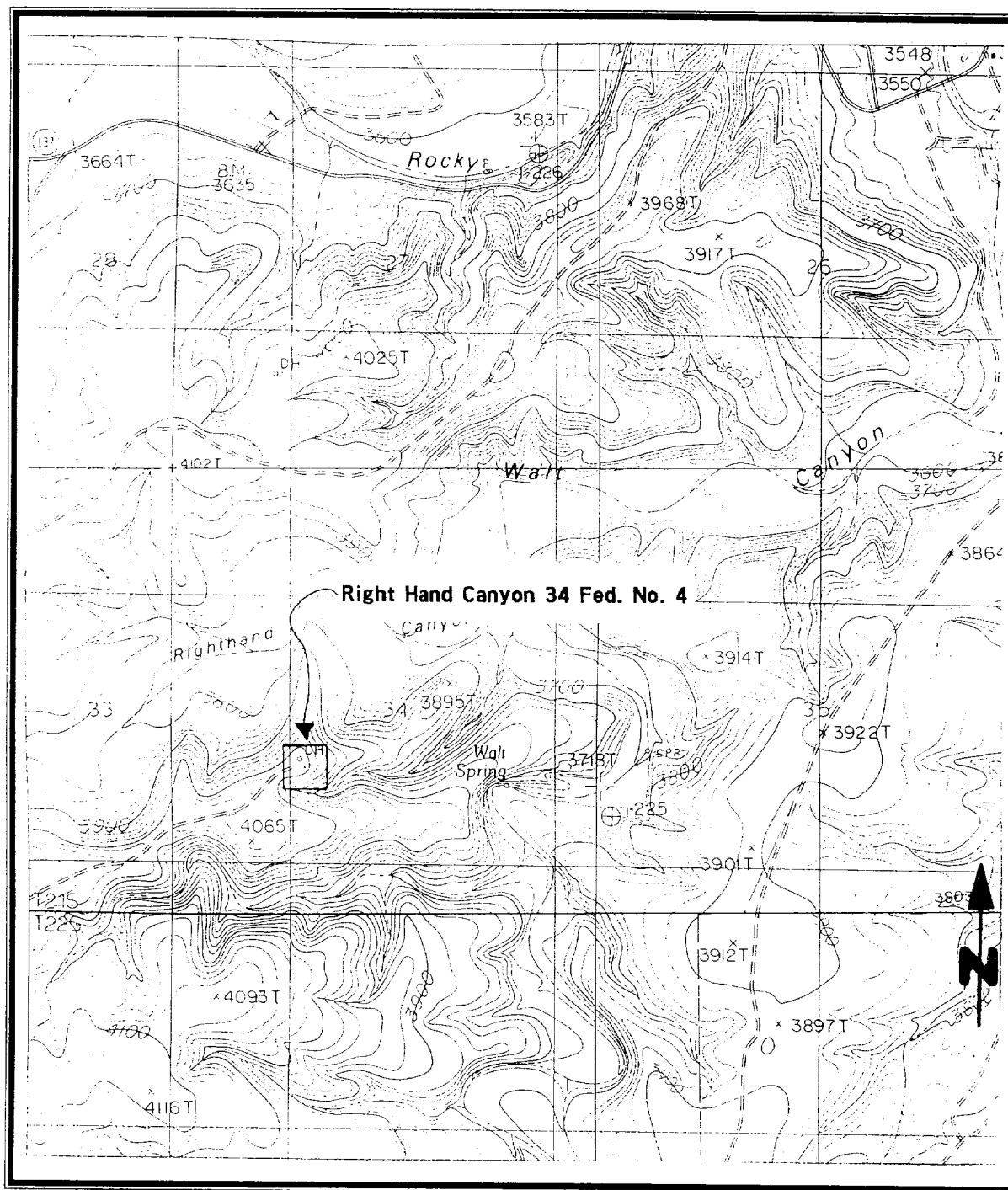
Figure 1. Survey Area Devon Energy Production Company, L.P. The Right Hand Canyon "34" Federal Number 4 Proposed Well Location Section 34, T.21S., R. 24E USGS Azotea Peak, NM 1985 7.5' topo map Eddy County, New Mexico Scale 1:24,000
