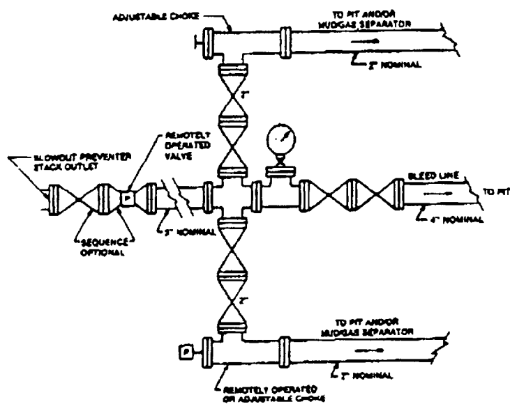
FIGURE K6.2. Typical choke manifold assembly for 3M rated working pressure service — surface installation.
