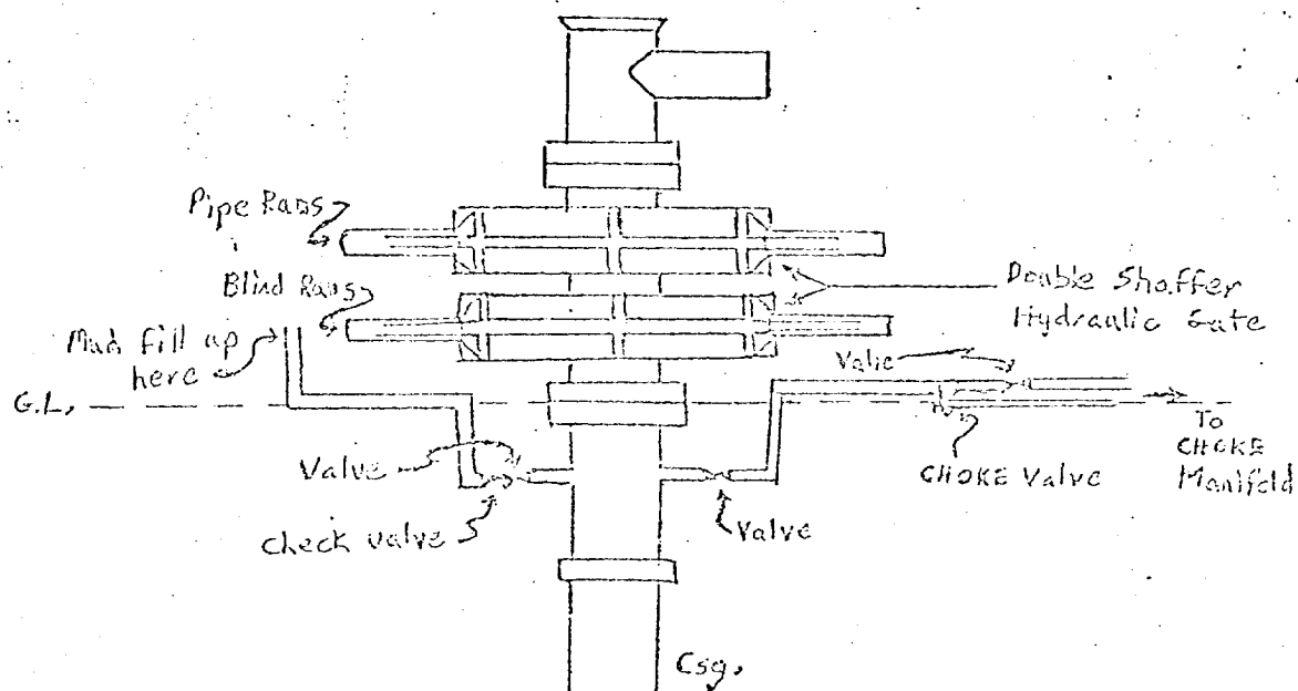
Blowout Preventor Diagram 10" x 900 Series MORANCO Rig #6 Adobe Oil Company Smith Federal No. 2 Section 11, T23S, R24E Eddy County, New Mexico
