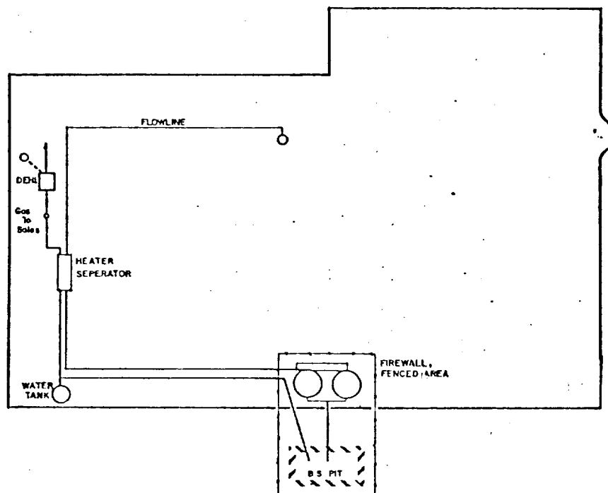
TANK BATTERY LAYOUT
