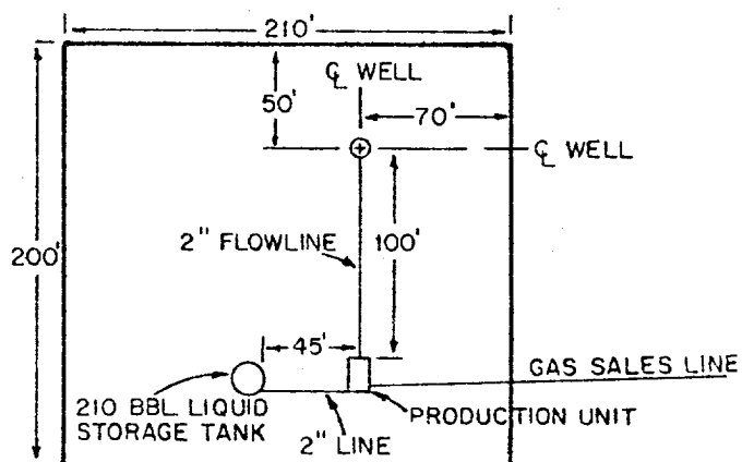
DETAIL of PRODUCTION FACILITIES SCALE: 1" = 100'
