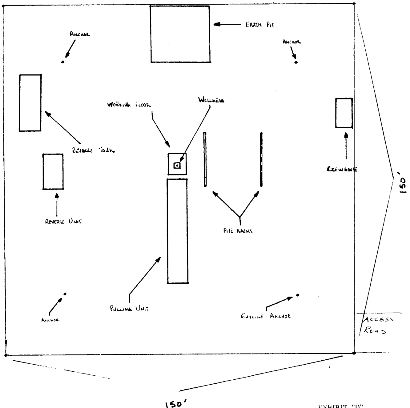
EXHIBIT "D" FUEL PRODUCTS, INC. Aspen Federal, Well No. 1 Pad & Pit Layout
