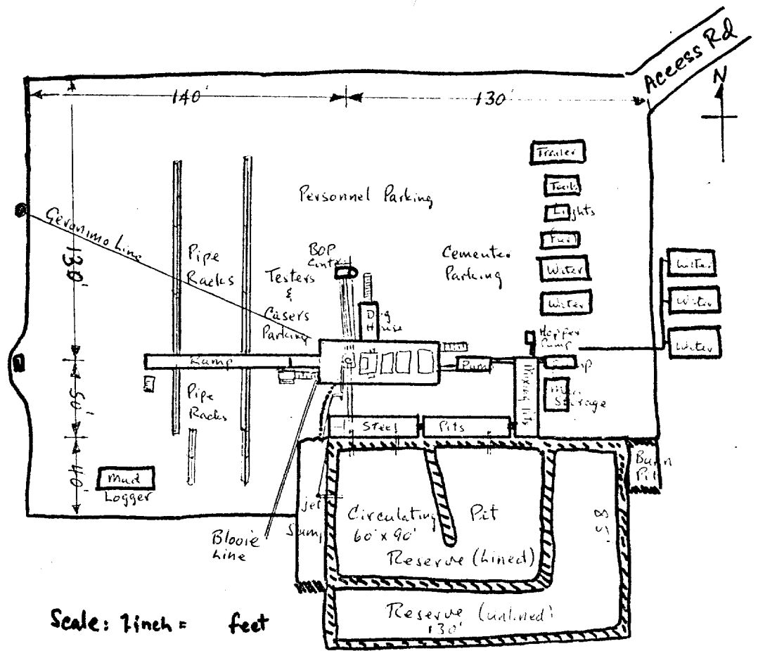
Drilling Rig layout
