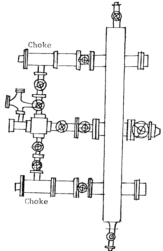
CHOKE & KILL MANIFOLD 4" X 2" 5000#
