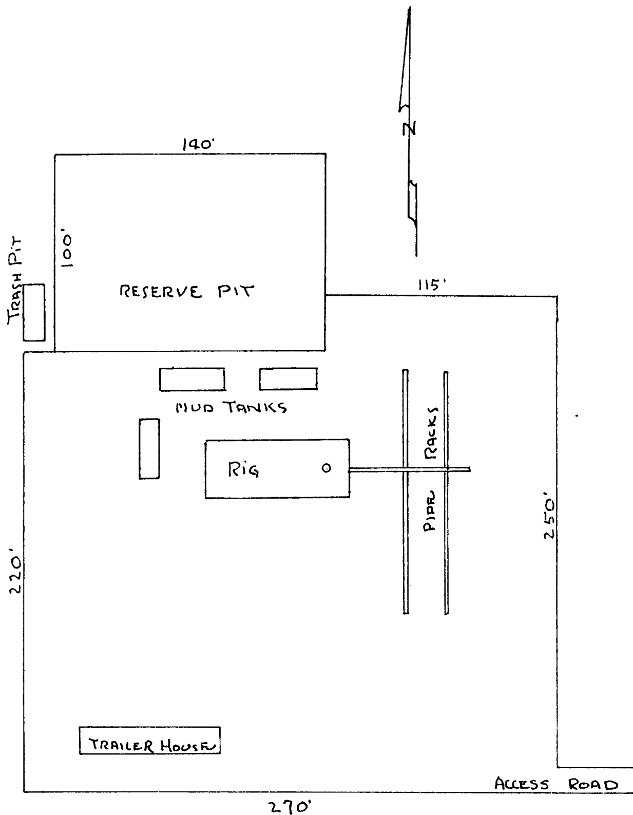
EXHIBIT "C" CORONADO EXPLORATION CORPORATION WELL NO. 1 CARTHEL FEDERAL SCALE: 1" = 50'
