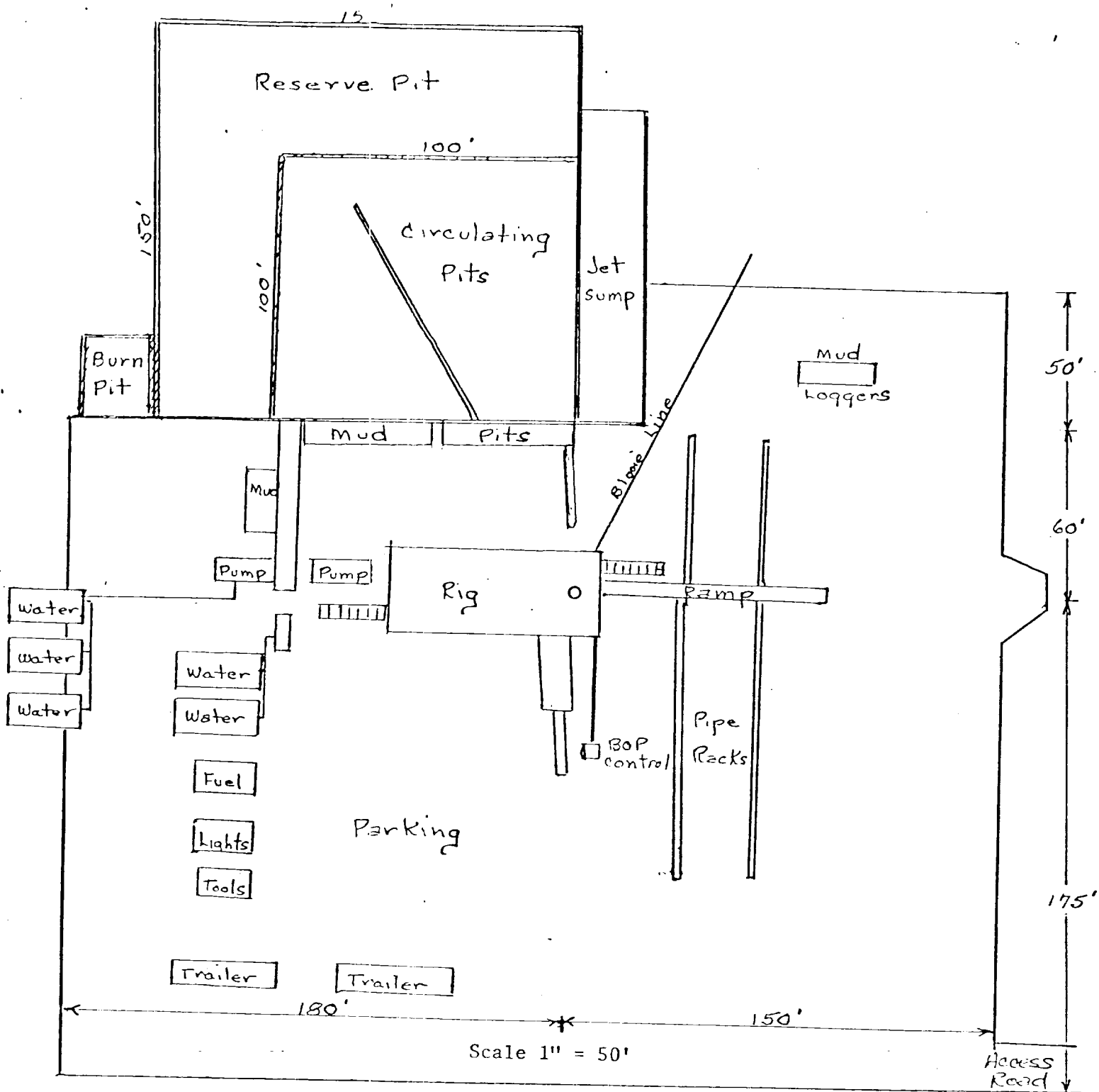
EXHIBIT D FORTSON FEDERAL COM. #1 Drilling Rig Layout
