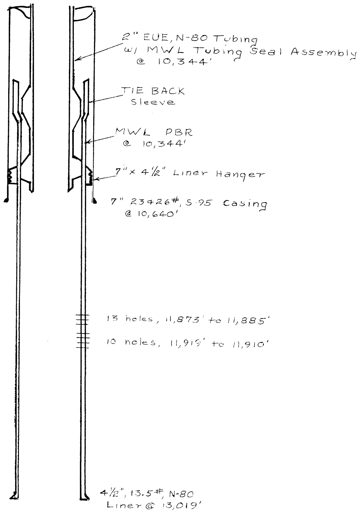
COMPLETION SCHEMATIC
