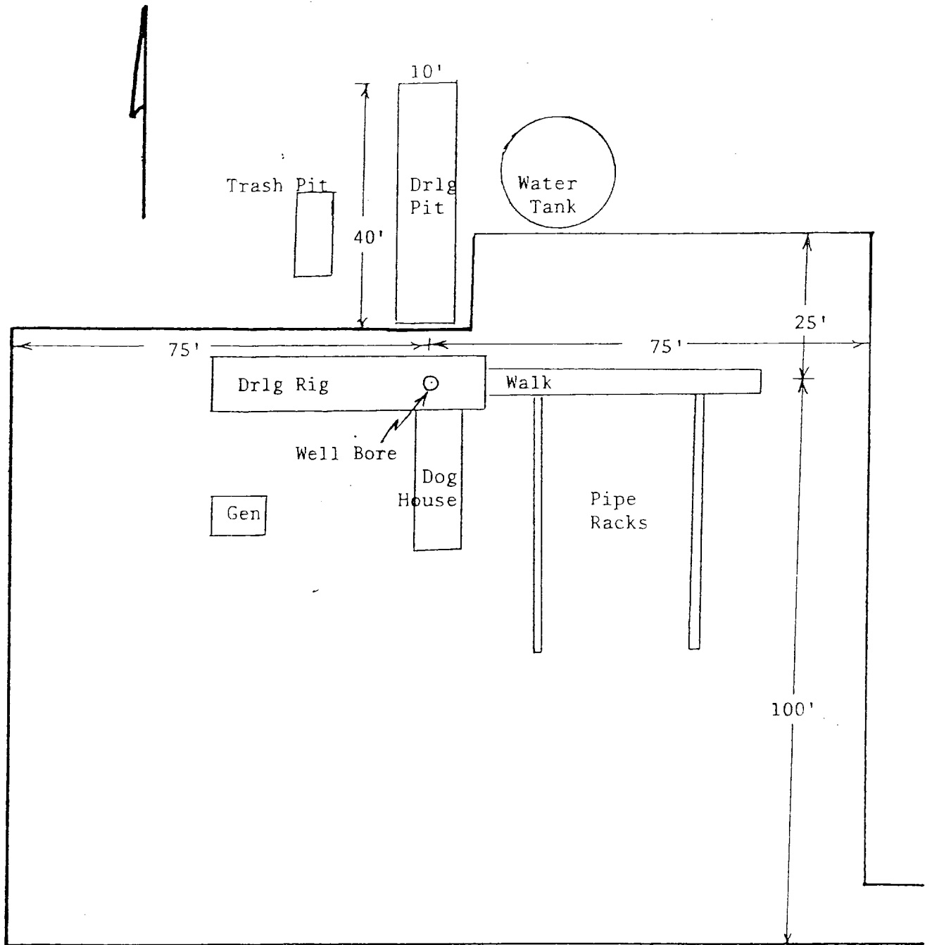
SUP Exhibit "D" SKETCH OF WELL PAD The Eastland Oil Company Avalon Federal Well No. 1 NE/4NE/4 Sec 7-24S-29E
