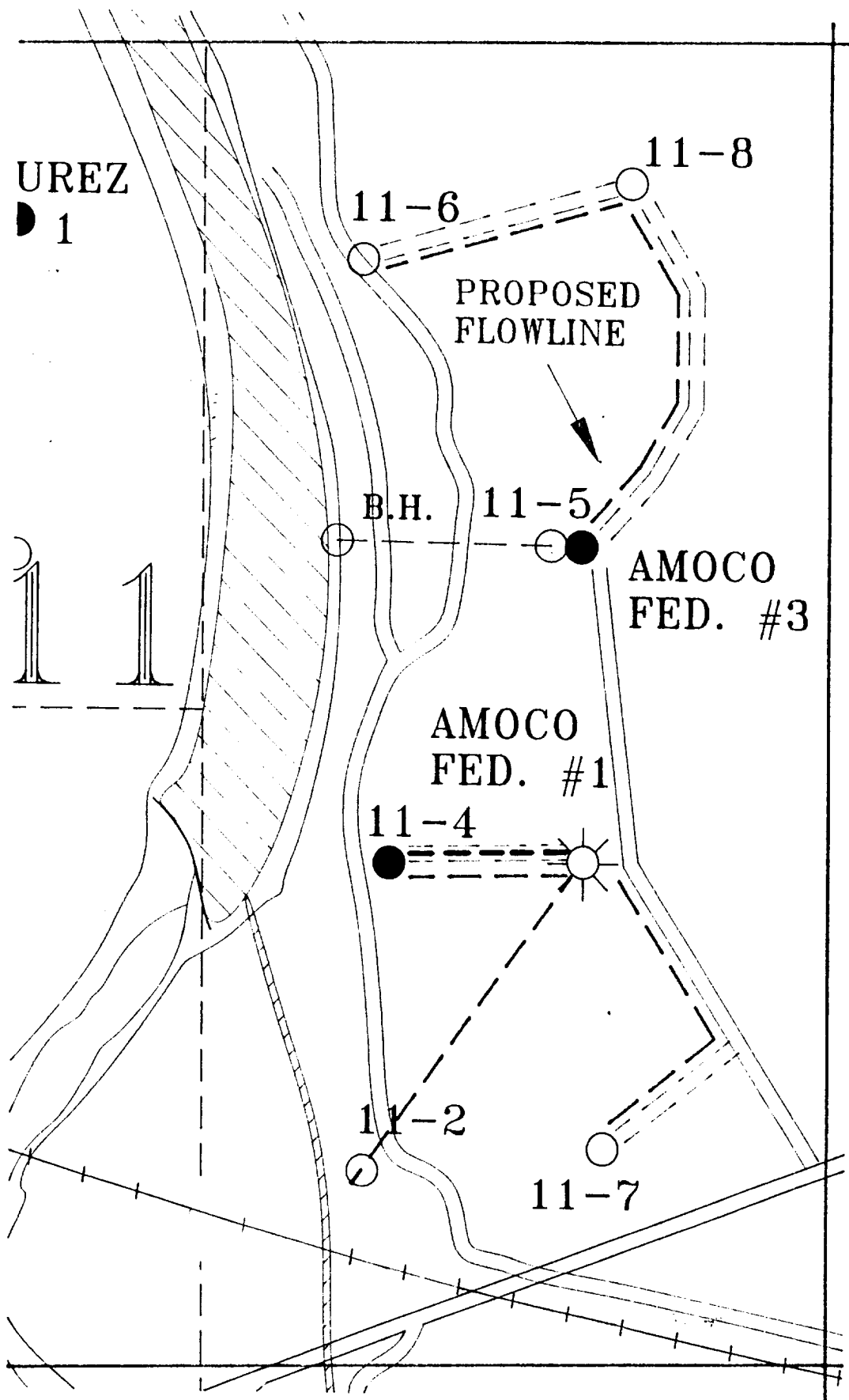
WELL: Amoco Federal #11-4 Road & Location Plat PLAT #6
