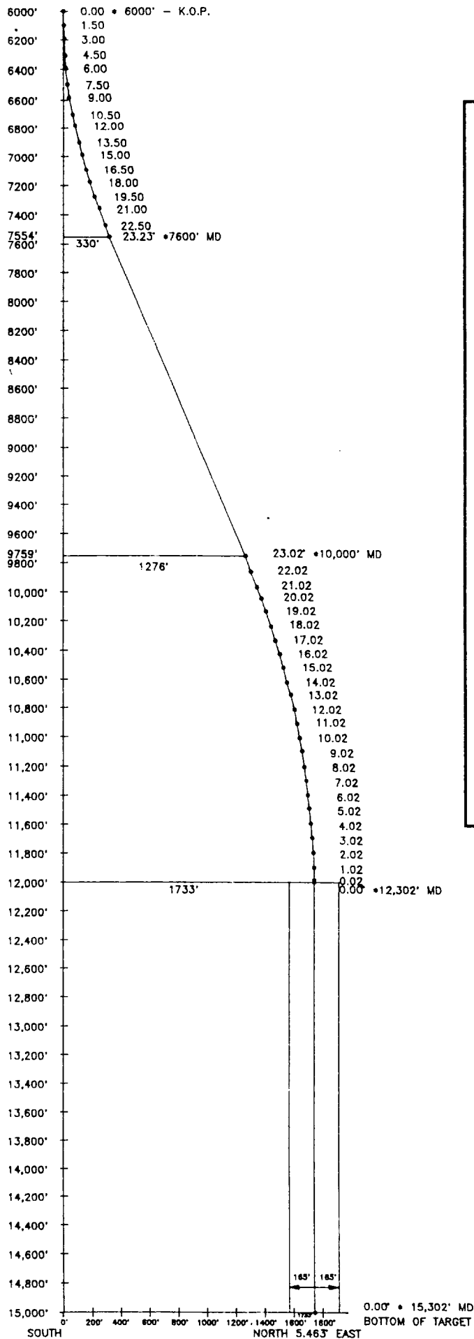
VERTICAL SECTION PLANE
