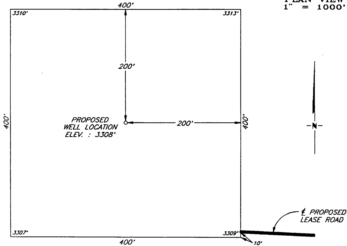
DETAIL VIEW 1" = 100'
