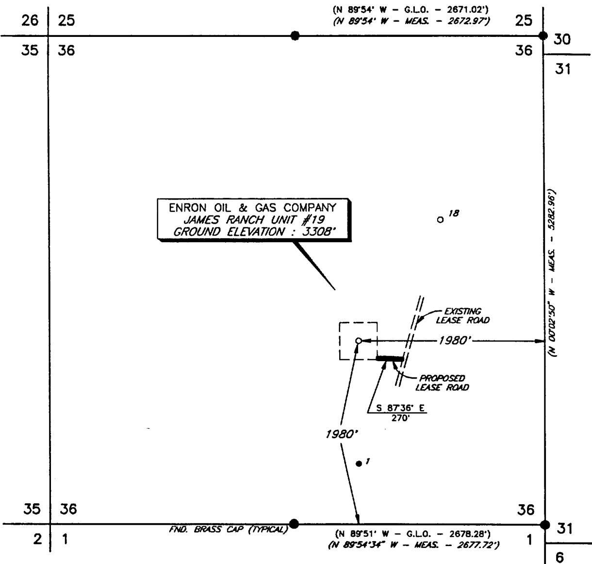
PLAN VIEW 1" = 1000'
