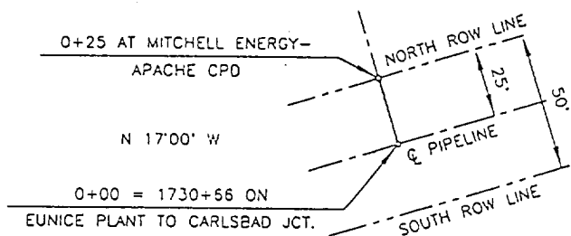
LINE DETAIL SCALE: 1" = 50'
