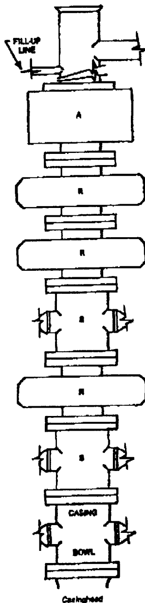
FIGURE K1-3. Recommended IADC Class 10 BOP stack arrangement SRSRRA, 10,000 psi WP, Lower drilling spool is optional with outlets on lower ram. 10,000 psi WP, 10,000 psi WP, 10,000 psi WP, 10,000 psi WP
