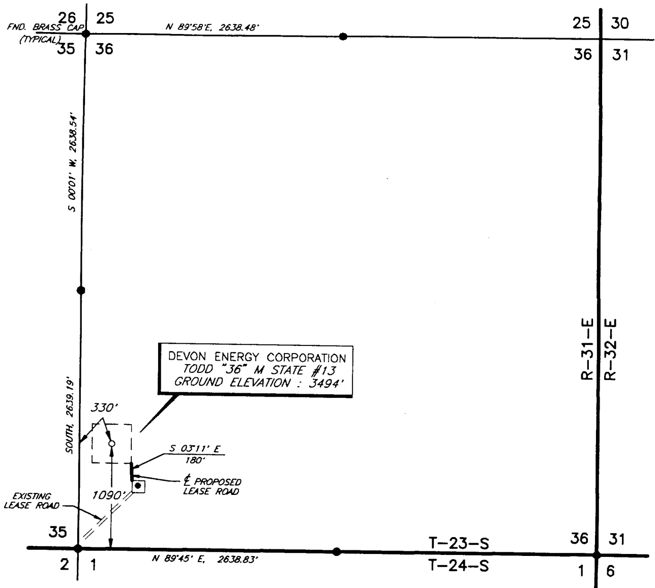
PLAN VIEW 1" = 1000'
