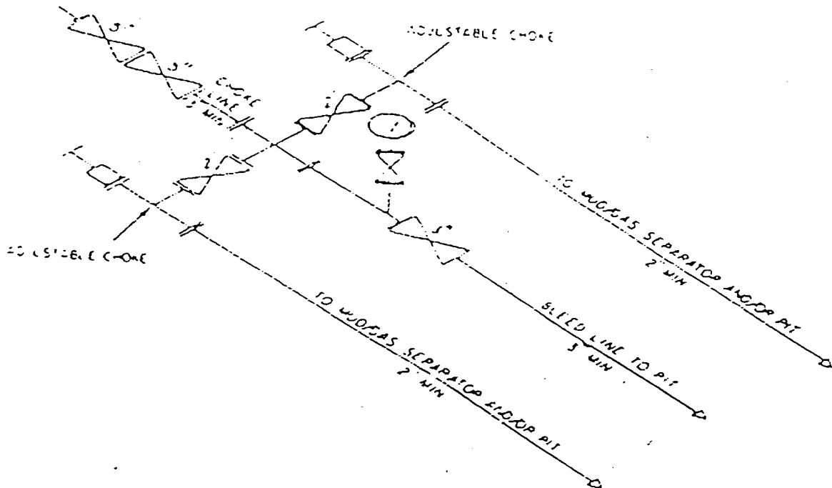
3M CHOKES MANIFOLD EQUIPMENT — CONFIGURATION MAY VARY
