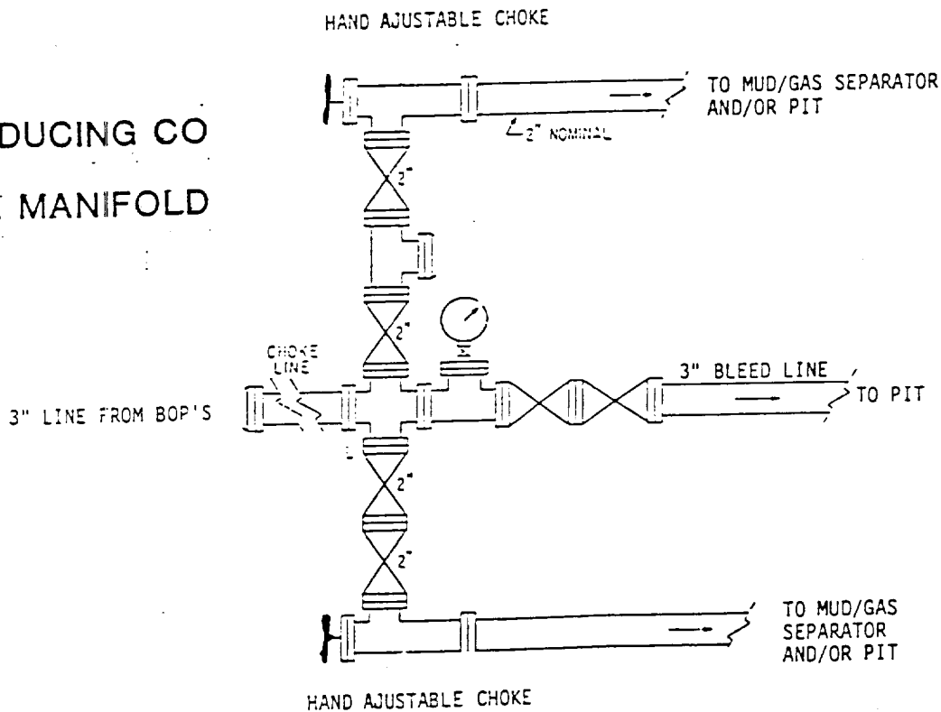
EXHIBIT "1-E" CHOKE MANIFOLD & CLOSING UNIT
