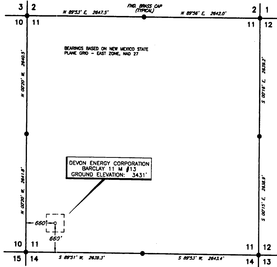
PLAN VIEW 1" = 1000'
