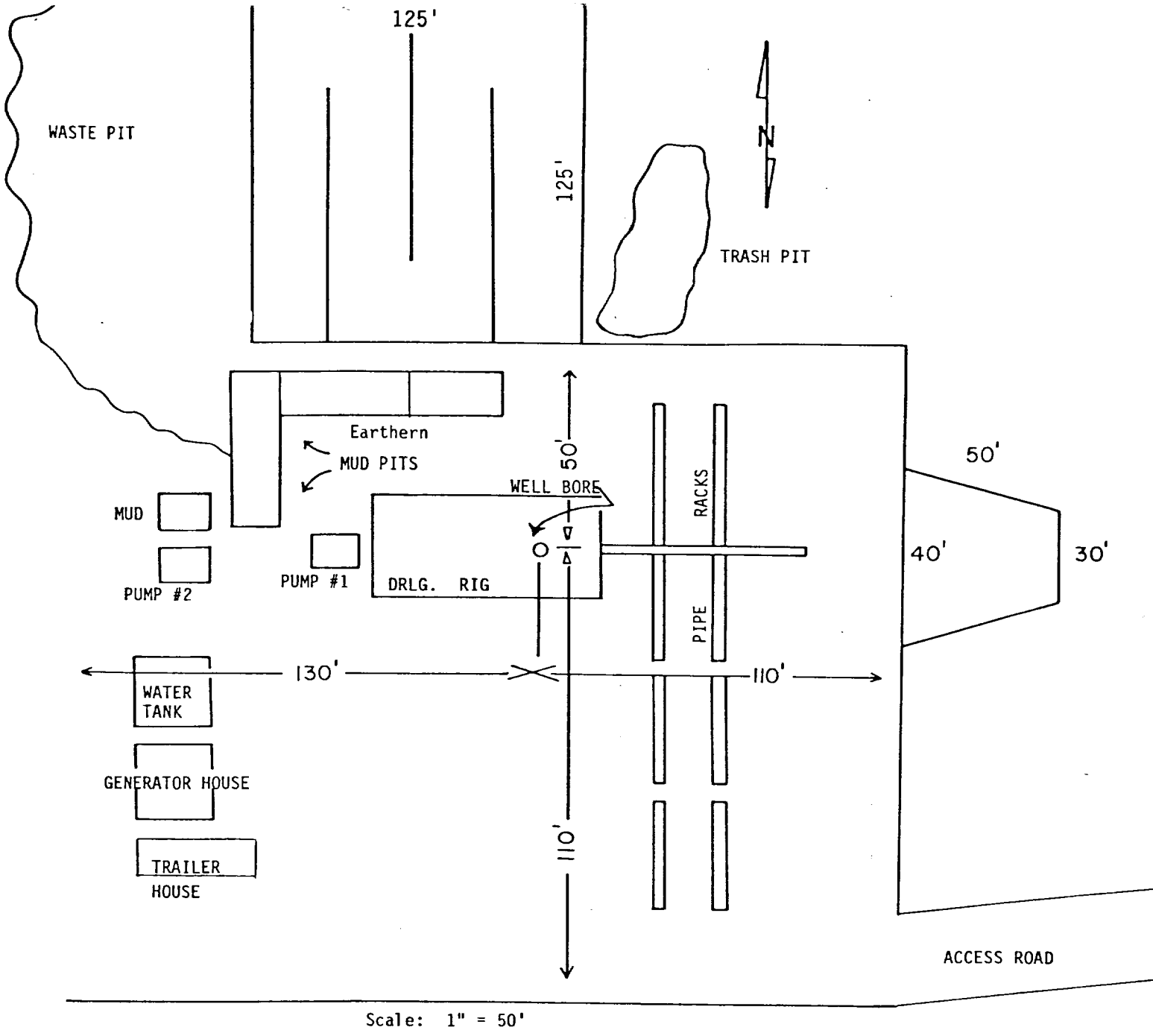
EXHIBIT "D" J.C. WILLIAMSON HOLLY "A" FEDERAL #6 DRILLING RIG LAYOUT
