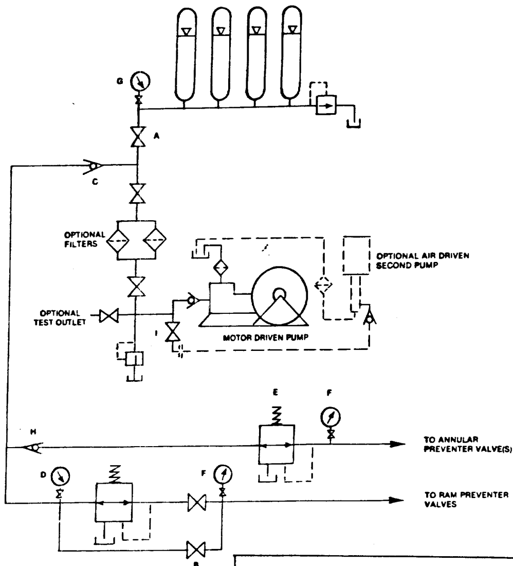
EXHIBIT E-1 Southwest Royalties, Inc. Choke Manifold & Closing Unit N. Brushy Draw "A" 35 Federal #3 Unit I 1980' FSL & 660' FEL, Section 35 T24S-R29E Eddy Co., NM.
