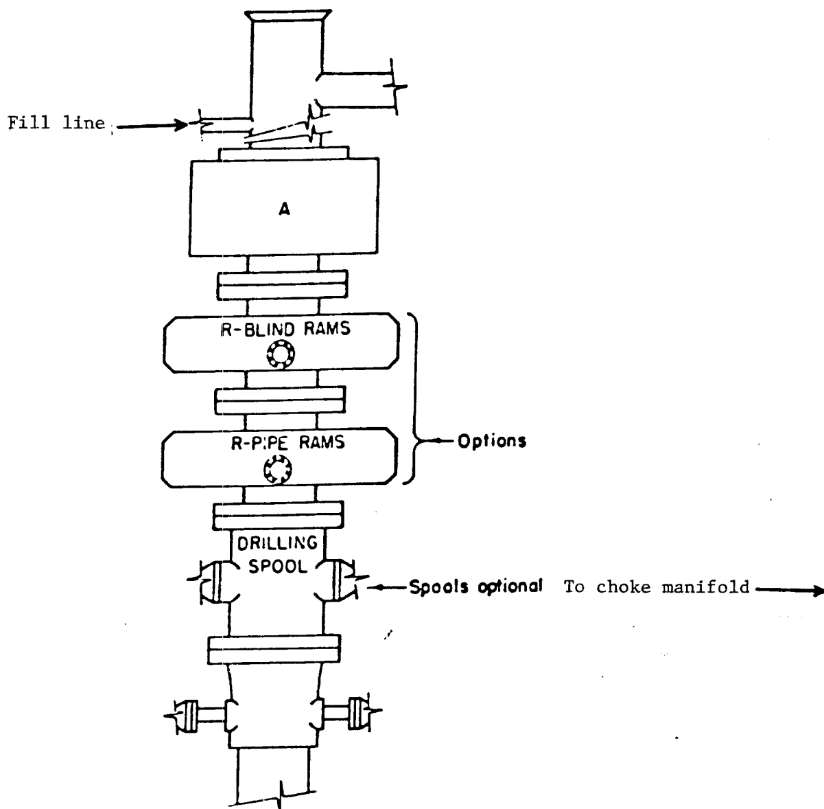
ARRANGEMENT SRRA
