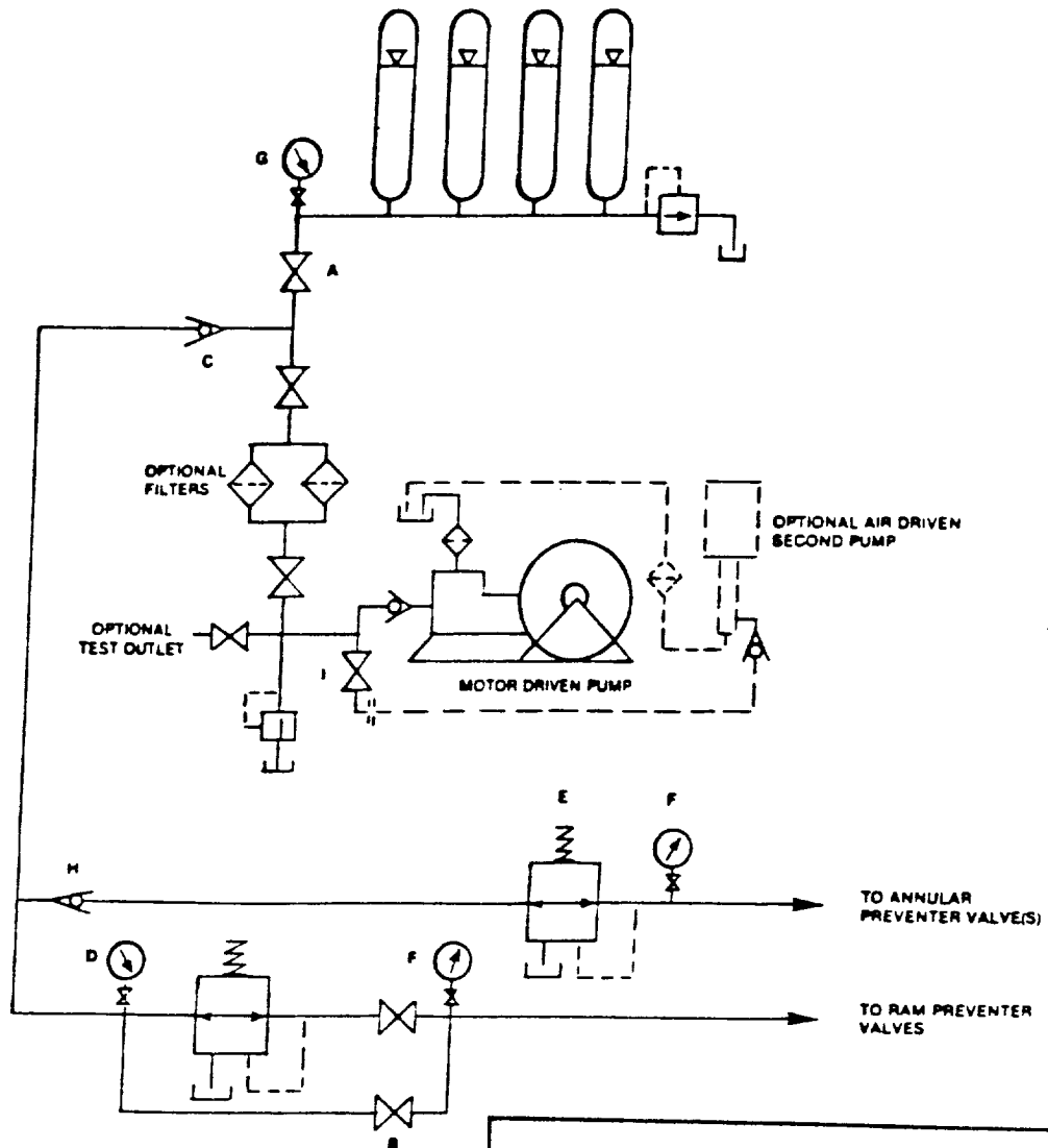
EXHIBIT E-1 SOUTHWEST ROYALTIES, INC. Choke Manifold & Closing Unit N. Brushy Draw "A" 35 Fed #8 Unit 0 660' FSL & 1980' FEL Section 35 T25S R29E Eddy Co., N.M.
