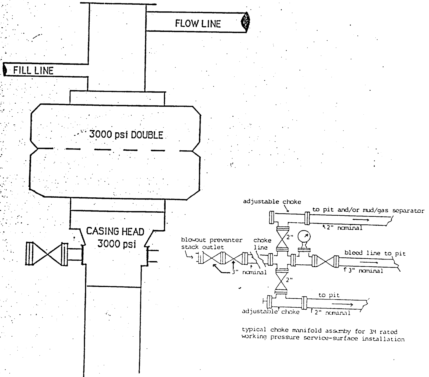
BLOWOUT PREVENTER 3M SYSTEM
