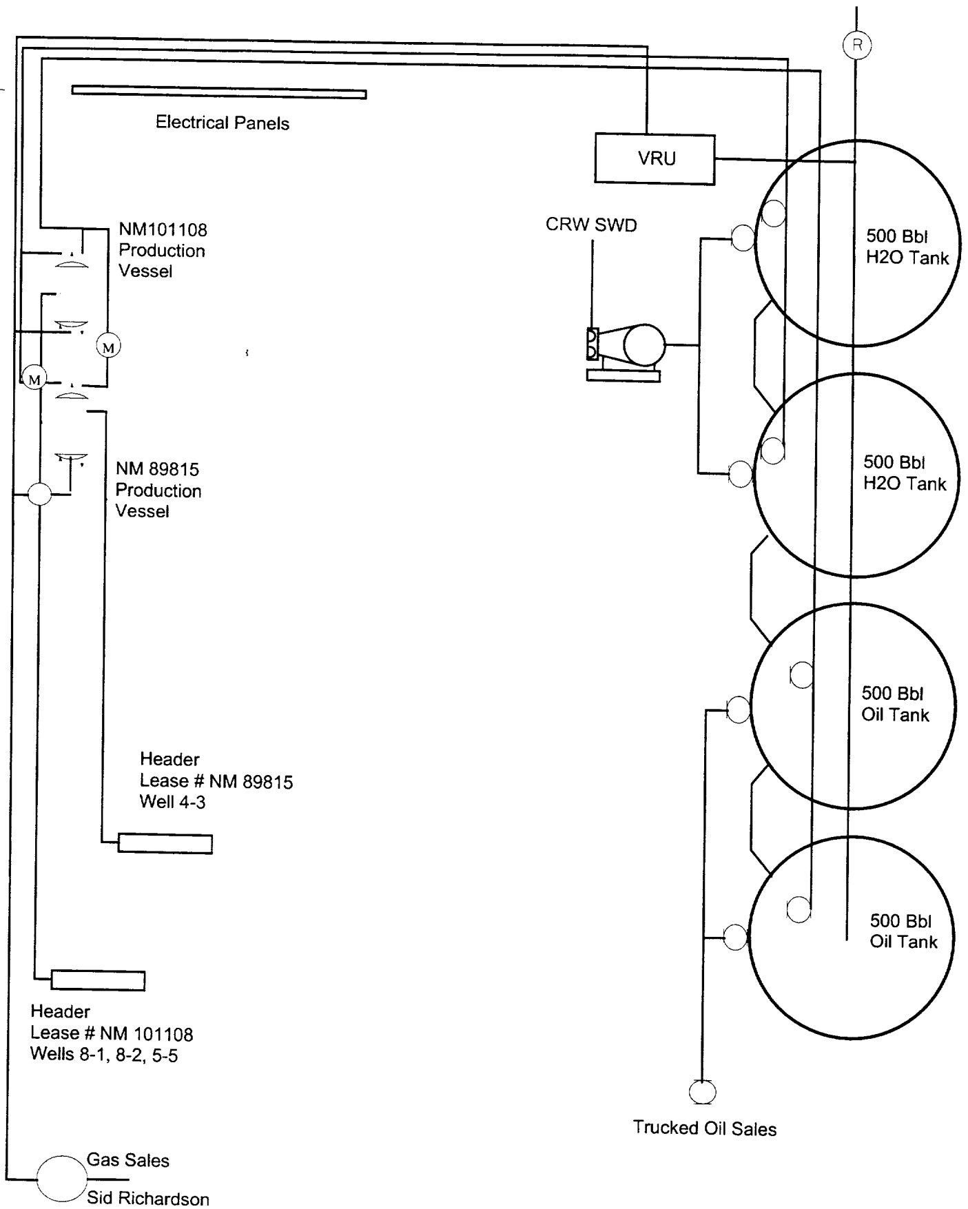
West Brushy Federal Battery Plot Plan
