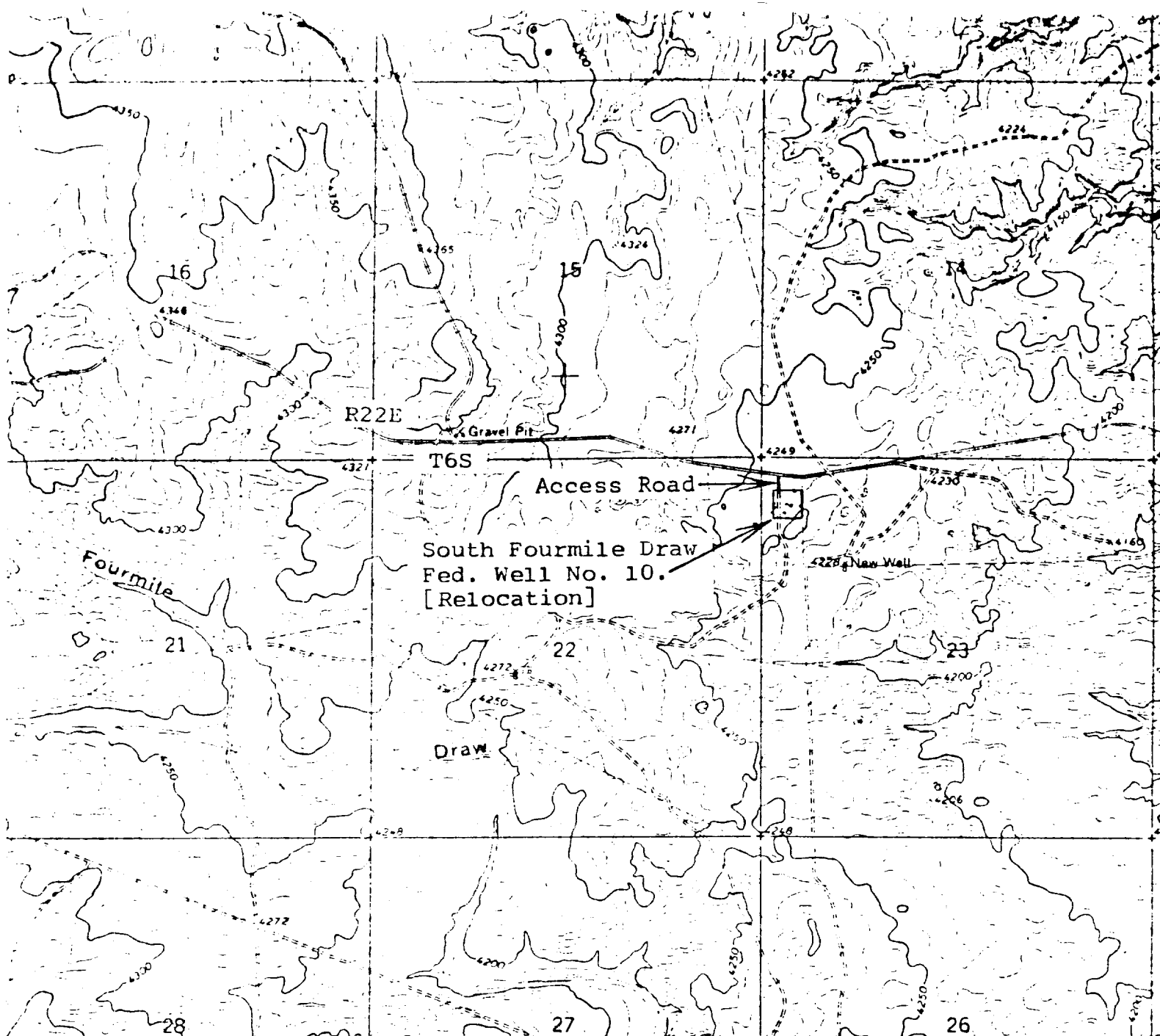
Map showing the location of the McKay Oil Corporation Relocation of the South Fourmile Draw Federal Well No. 10 and access road. T6S, R22E, Section 23, Centre, W1/2, NW/4NW/4 [660 FNL, 330 FWL], Chaves County, New Mexico. Square shows location of well pad; solid line shows location of access road; dots show location of Isolated Finds. U.S.G.S. 7.5 minute series, MESA SW, NEW MEXICO, 1967, photorevised 1982. ASC project: 87-75.
