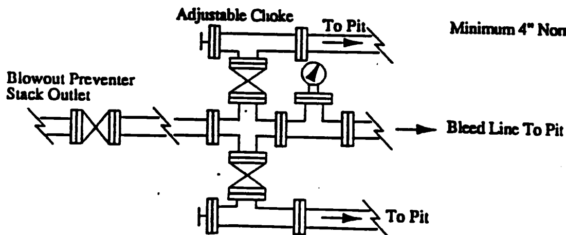
Choke Manifold Requirement ( 3000 psi WP)
