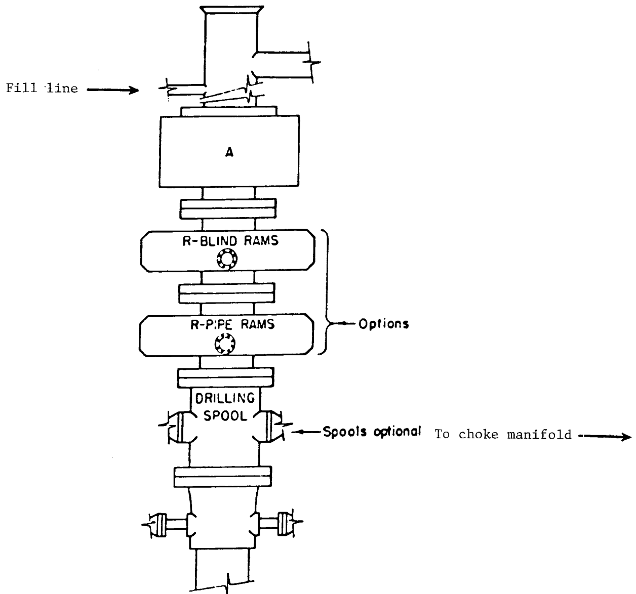
ARRANGEMENT SRRA
