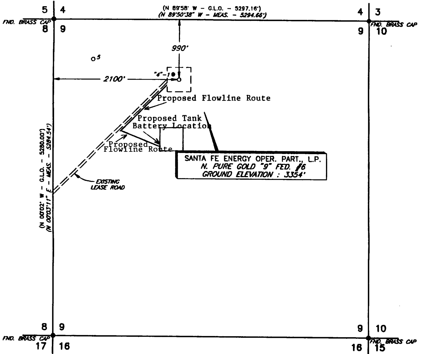
PLAN VIEW 1" = 1000'
